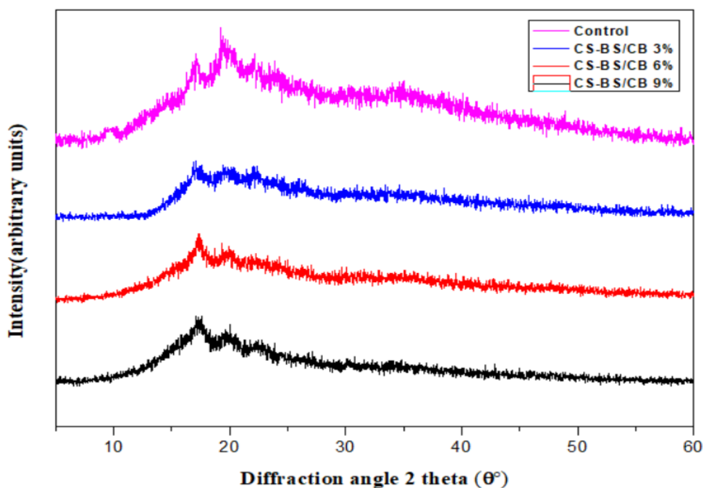
Figure 3. X-ray diffraction curves of black seed/cassava bagasse fiber reinforced cornstarch hybrid composite film.
