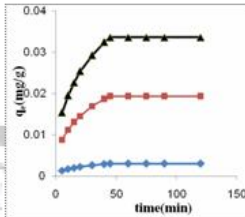
Fig.(7): Effect of initial concentration onto adsorption of (10, 25 and 40)mg/L of thymol solution
