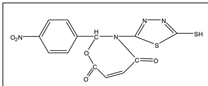
Figure (1): The structure of 1,3-oxazepine derivative(15)
