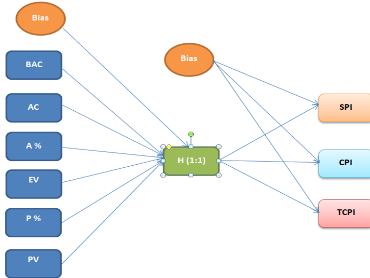
Figure. 1 Architecture of ANN model
