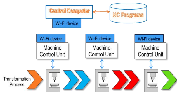
Figure 1. Wireless Controller System.
