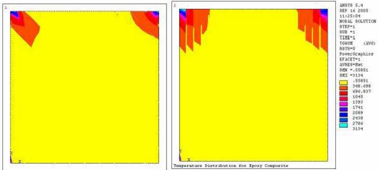
(b) (a) Thermal gradient for Epoxy Composite [(a)- 0°, (b)- 45°]
