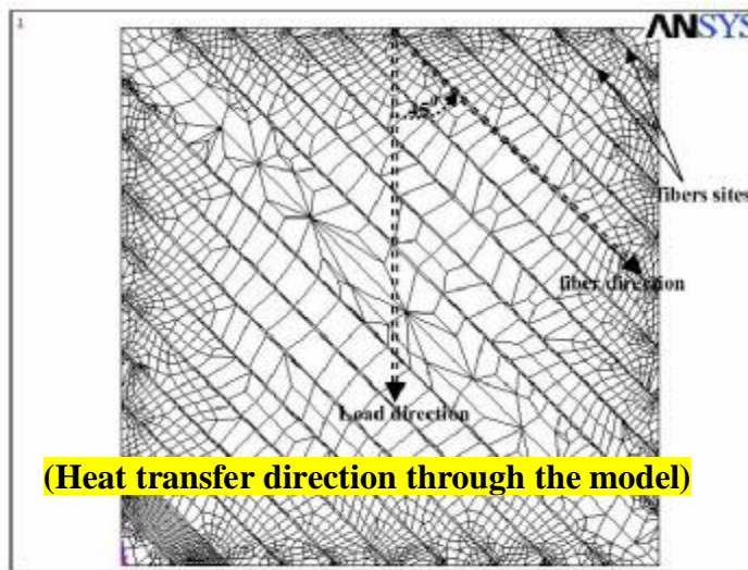
Fig (2-b) finite element mesh, fibers angled at 45^{\circ} with the load direction
