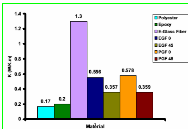
Fig(7) Thermal conductivity for all studied materials
