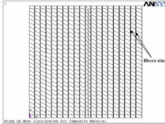
Fig (2-a) finite element mesh, fibers angled at 0^{\circ} with the load direction
