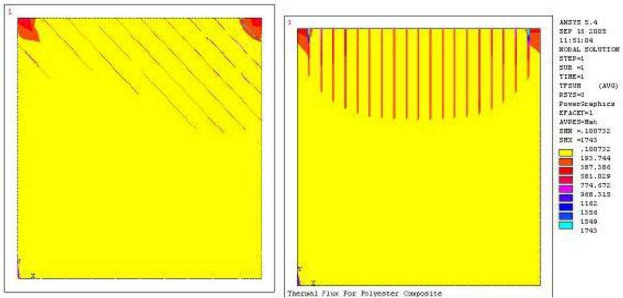
(b) (a) Thermal flux for Epoxy Composite [(a)- 0 o , (b)- 45 o ]
