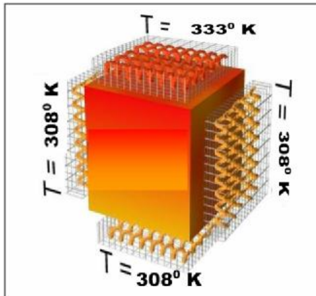
fig(3) Virtual simulation for the boundary conditions applied to the models
