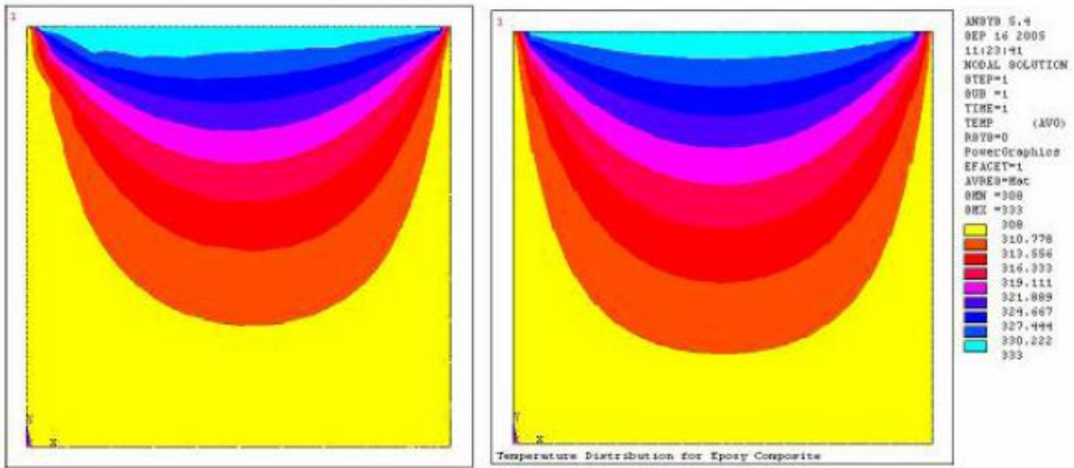
(b) (a) Temperature distribution for Epoxy Composite [(a)- 0^\circ , (b)- 45^\circ ]
