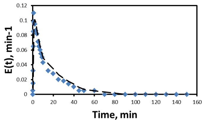
Figure 9 Age function and residence time distribution (experimental data; ----- ◆ fitted data using the mixing with dead time model).
