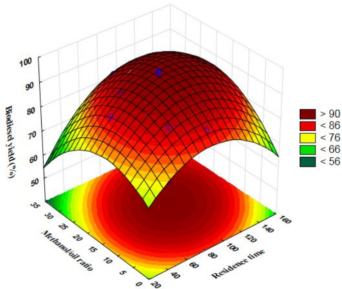
Figure 4 Influence of methanol/oil ratio and residence time on biodiesel yield: reaction temperature 368.15 K; catalyst loading 8 wt%.
