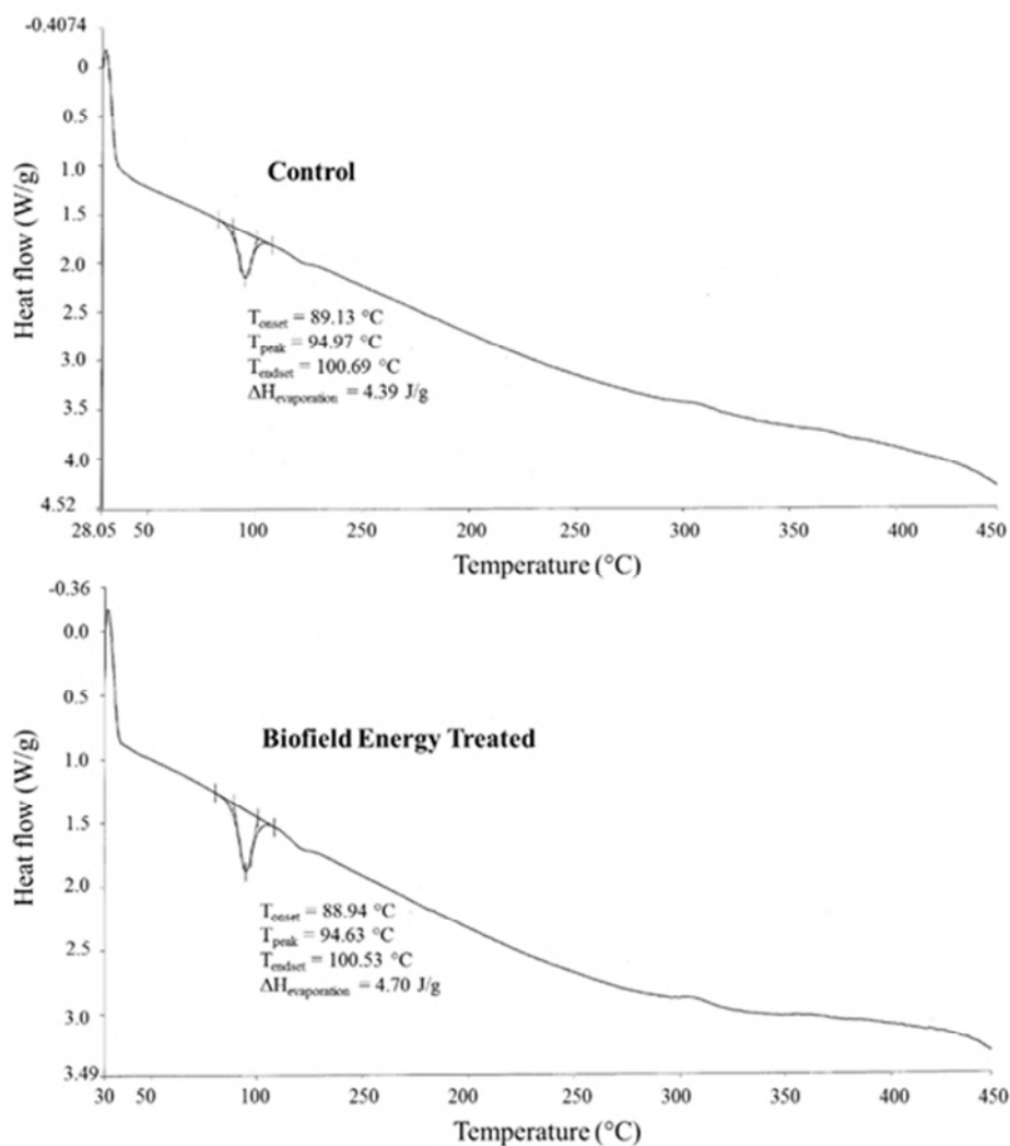
Figure 5. DSC thermograms of the control and Biofield Energy Treated sodium selenate.
