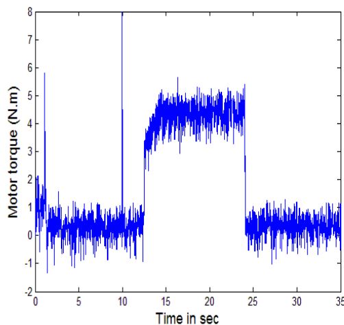
Fig.29 The estimated motor torque with classical method
