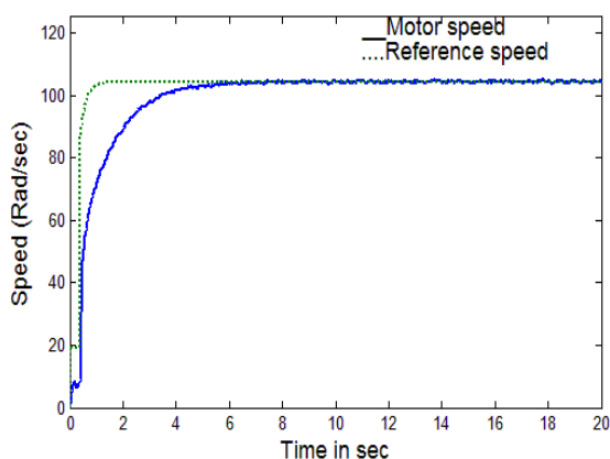
Fig.25 The motor speed with classical method
