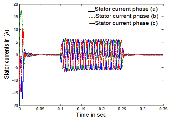
Fig.18 The motor current with modified method
