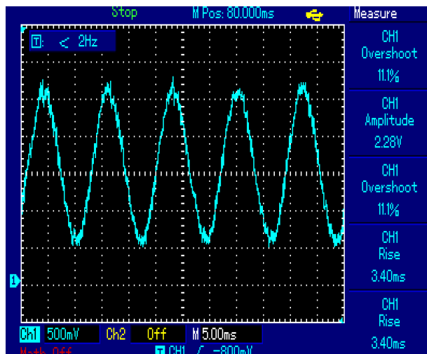
Fig.28 The motor current with modified method
