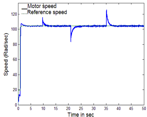
Fig.36 The motor speed with classical method when fourth PI was used
