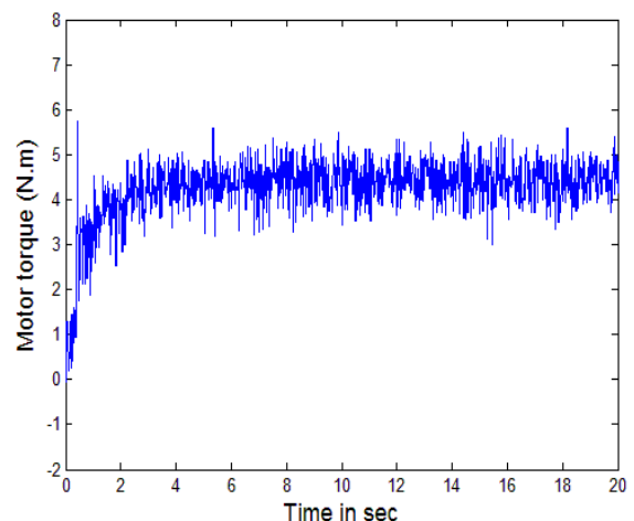
Fig.23 The estimated motor torque with classical method
