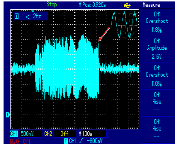
Fig. 34 The motor current with modified method
