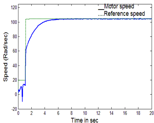
Fig.26 The motor speed with modified method
