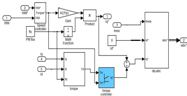
Fig. 4 VC details for classical and modified methods in case of sudden applied or removal the load
