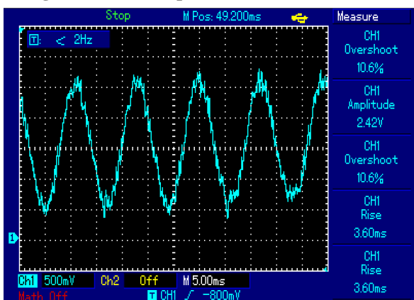
Fig.27 The motor current with classical method
