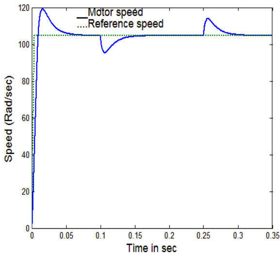
Fig.15 The motor speed with classical method
