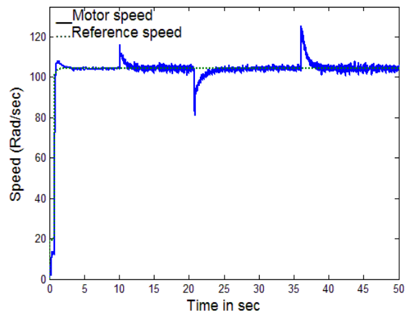
Fig. 35 The motor speed with classical method when fourth PI was used
