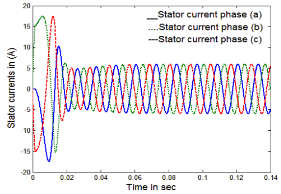
Fig.12 The motor current with modified method
