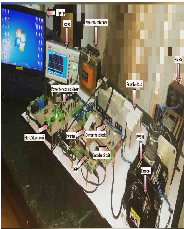
Fig. 22 A Photo Lab
