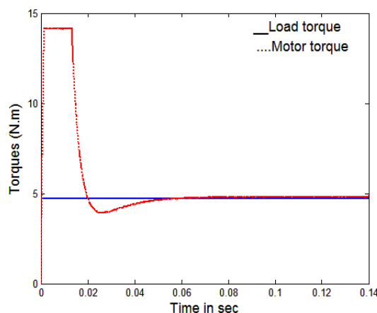
Fig.8 The torque with modified method
