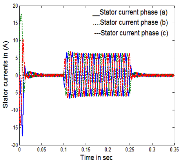
Fig.17 The motor current with classical method
