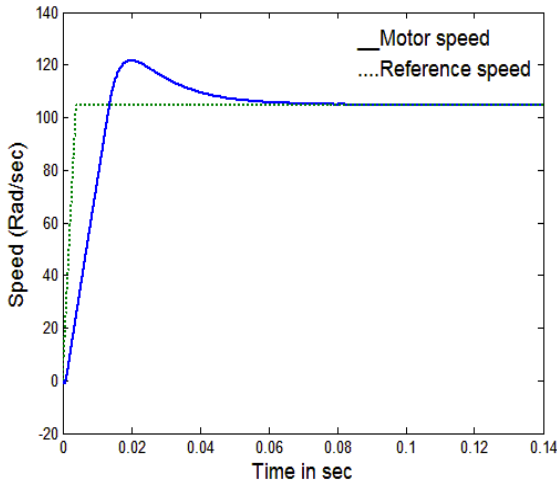
Fig.9 The motor speed with classical method
