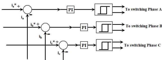
Fig. 6 Modified current regulated block.
