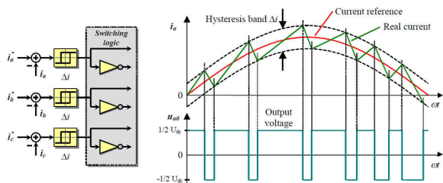
Fig. 5 Hysteresis PWM current control and switching logic
