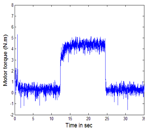
Fig.30 The estimated motor torque with modified method
