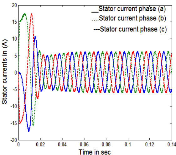
Fig.11 The motor current with classical method
