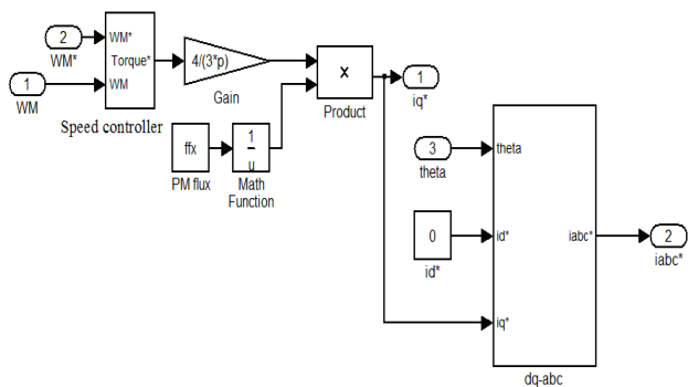
Fig. 3 VC details for classical and modified methods
