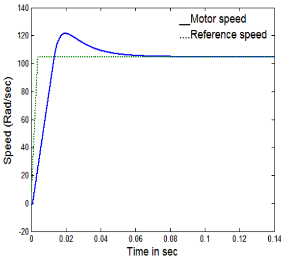
Fig.10 The motor speed with modified method
