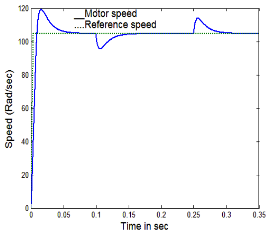
Fig.16 The motor speed with modified method
