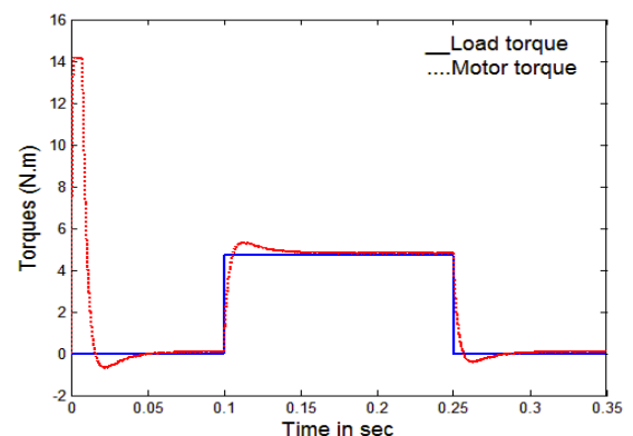
Fig.14 The torque with modified method
