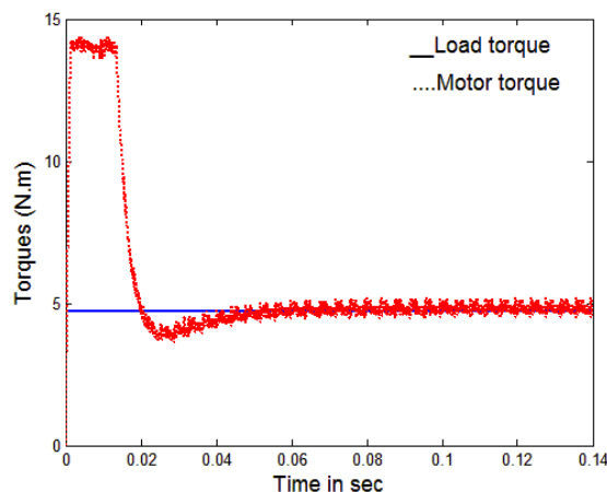
Fig.7 The torque with classical method
