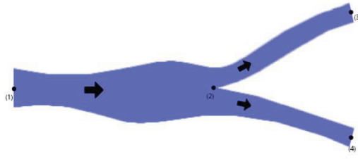
FIGURE 3. Irregular Fractal.
