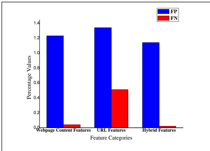
Fig.3: Prediction sensitivity in terms of the category of features space, and percentages of FP and FN.
