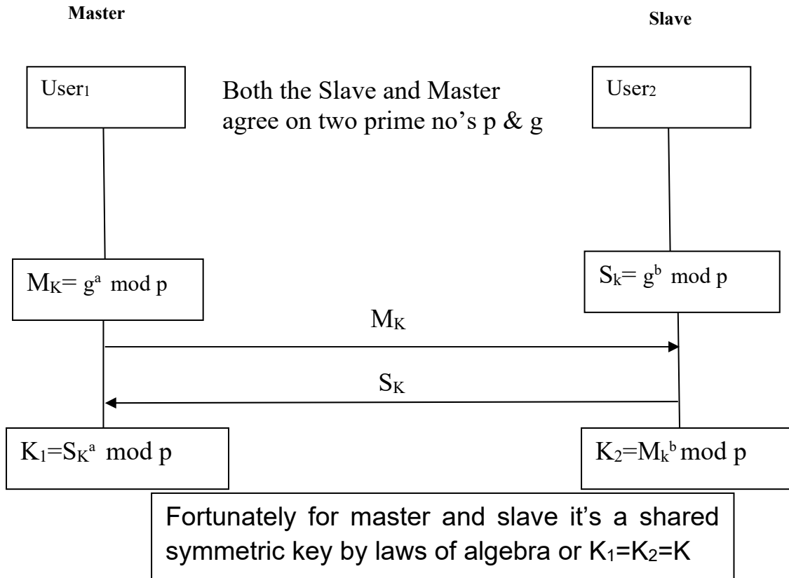
Fig(5): Diffie-Hellman Key exchange
