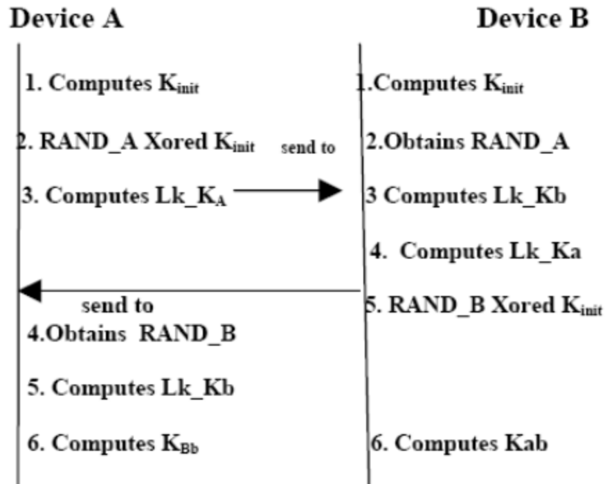
Fig. (4) Bluetooth coupling Mechanism
