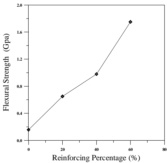
Fig(5): Flexural Strength
