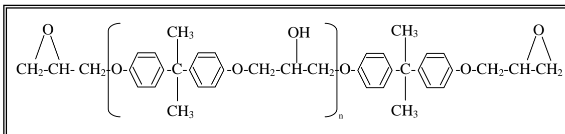
Figure (1): Chemical structure of Araldite resin [Mallick,2007]
