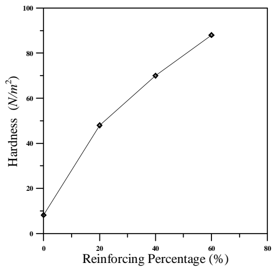
Fig(6): Hardness
