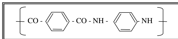
Figure (2): Chemical structure of kevlar fibers[Mallick,2007]
