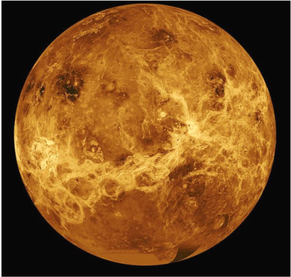
VENUS -THE MORNING STAR- RADAR IMAGE
