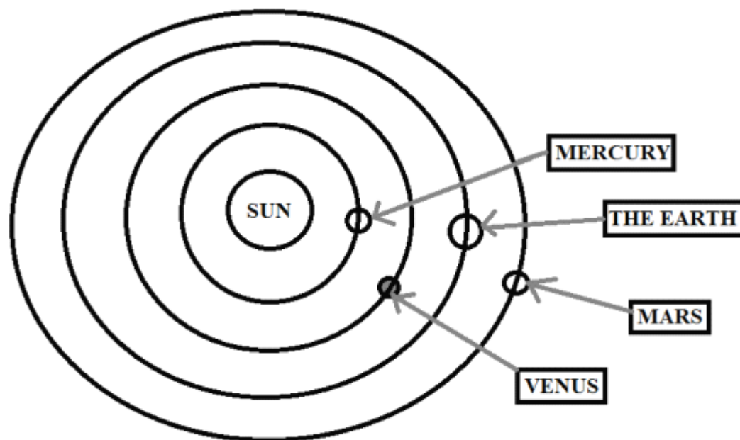
FIG. : REPRESENTS THE SUN, MERCURY, VENUS, THE EARTH , AND MARS PLANETS IN NOT TRUE SCALE.
