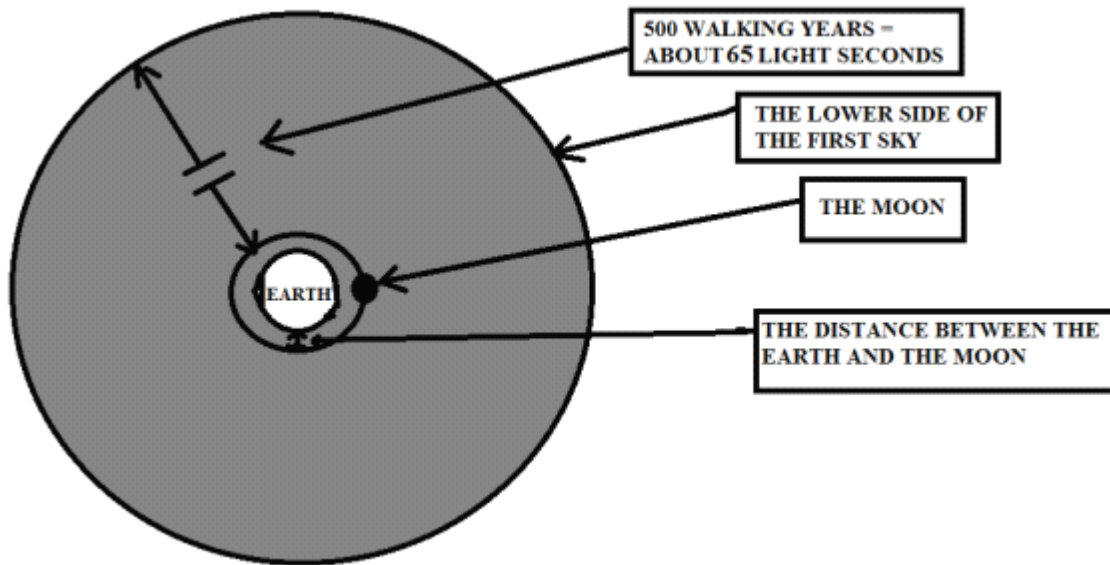
FIG. EXPLAIN THE LOCATION OF THE MOON
