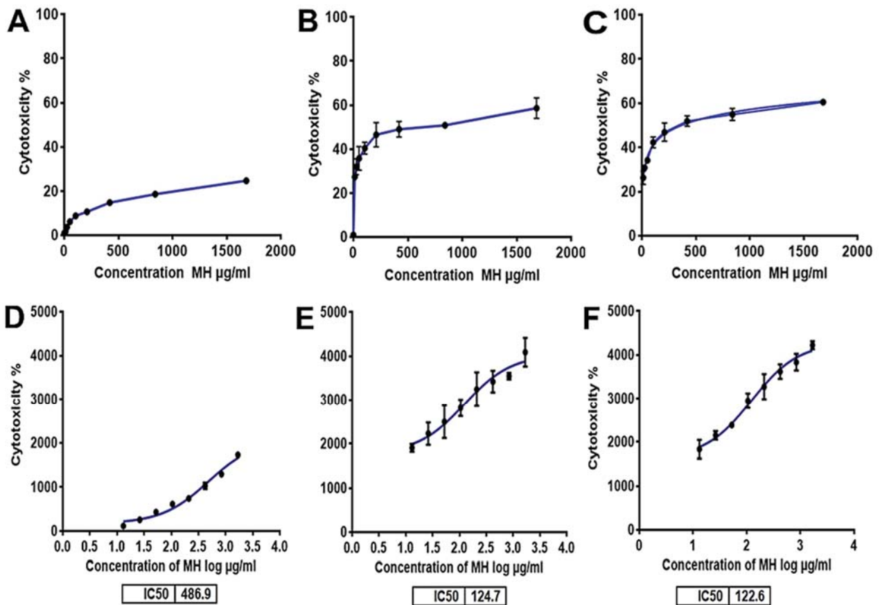
FIGURE 1. Cytotoxicity (%) of different concentrations of D-mannoheptulose (MH) to A- REF, B- AMJ13, and C- MCF7 cells. IC 50 of MH on D- REF, E- AMJ13, and F- MCF7 cells as computed by the GraphPad Prism program.
