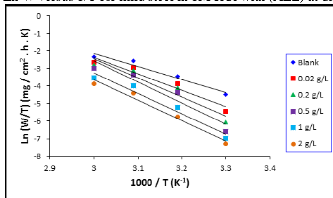
Figure 10: Arrhenius plots of Ln (W/T) versus 1/T for mild steel in 1M HCl with (AEGPD) at different concentrations.
