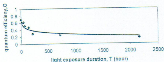
Figure 7: Quantum efficiency as a function of light exposure duration
