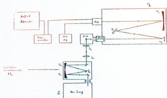
Figure 4: The Fluorescence Measuring System
