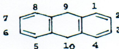
Figure 1: Anthracene Molecule
