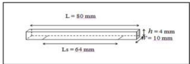
Figure 3: ASTM (D790).
