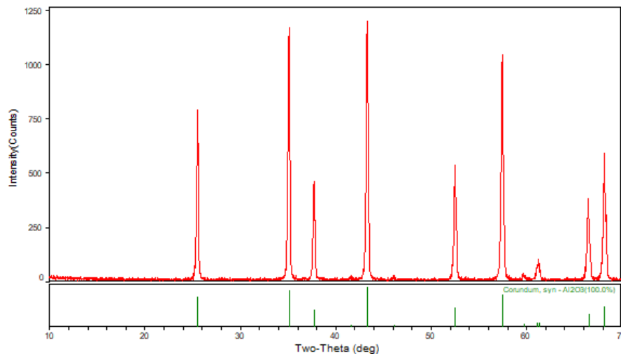
FIGURE 3 XRD pattern of alumina powder calcined at 1200°C for 2 hours with a heating rate of 5°C/min
