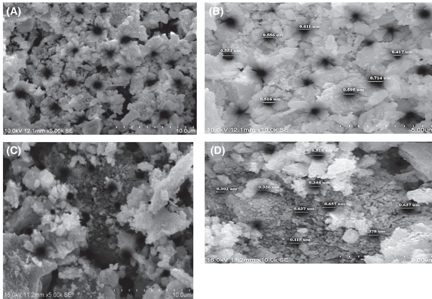
FIGURE 5 SEM of (A) sample with 20wt% and sintering at 1200°C at 5.0KX, (B) sample with 20wt% and sintering at 1200°C at 10.0KX, (C) sample with 20wt% and sintering at 1500°C at 5.0KX, (D) sample with 20wt% and sintering at 1500°C at 10.0KX
