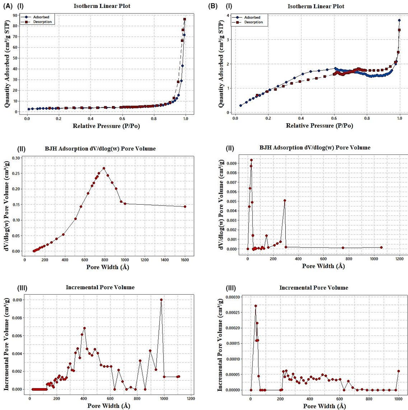
FIGURE 6 BET result of porous alumina (A1, A2, A3) of sample with 20wt% and sintering at 1200°C, (B1, B2, B3) of sample with 20wt% and sintering at 1500°C
