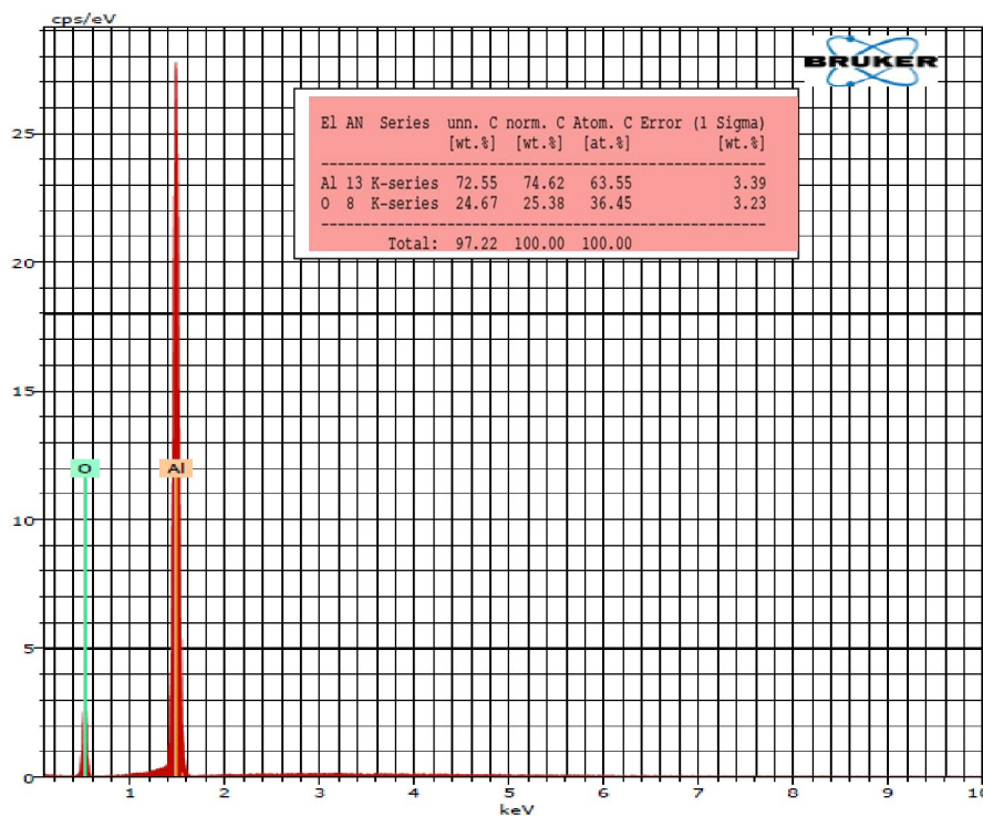
FIGURE 4 EDS analysis of alumina powder
