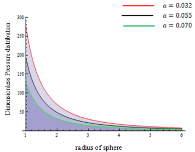
Figure 2. Variation of dimensionless pressure distribution with radius of sphere for different values of elastic deformation
