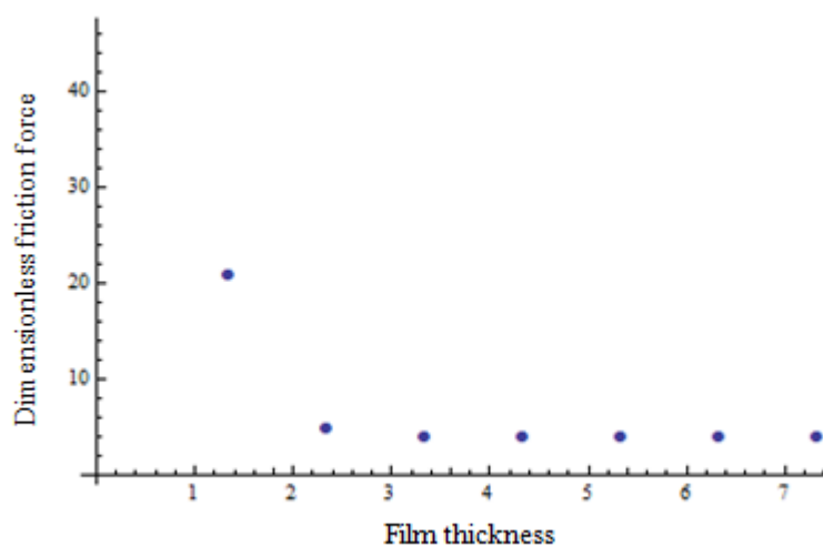
Figure 9. Relationship between dimensionless friction force and film thickness of type lubrication
