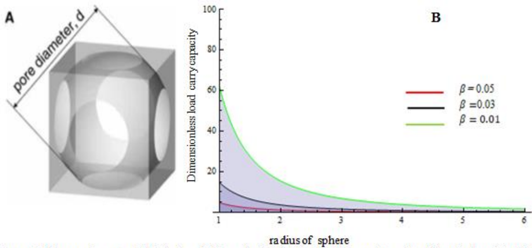
Figure 6 (A) pore diameter (B) Variation of dimensionless load carrying capacity with radius of sphere for different values of pore size
