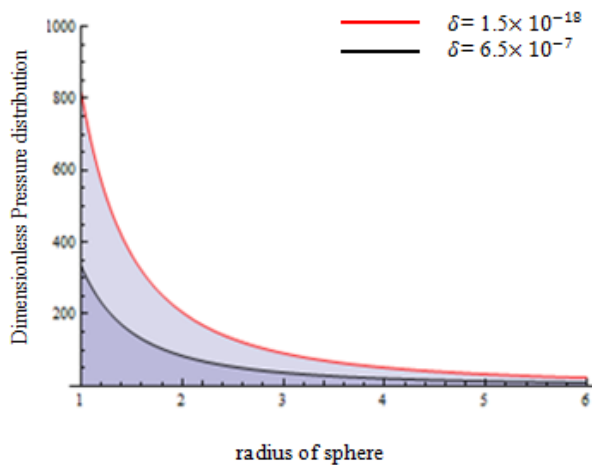
Figure 3. Variation of dimensionless pressure distribution with radius of sphere for different values of permeability
