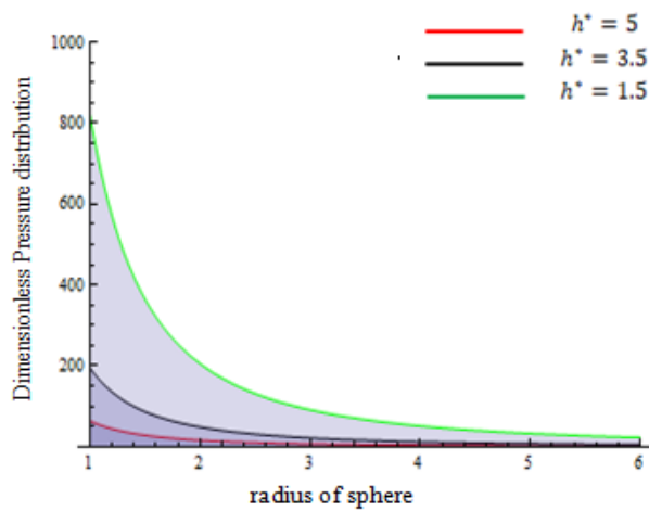
Figure 1. Variation of dimensionless pressure distribution with radius of sphere for different values of film thickness
