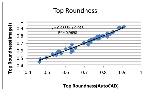
(a) top Roundness Index
