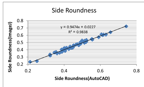
(b) side Roundness Index
