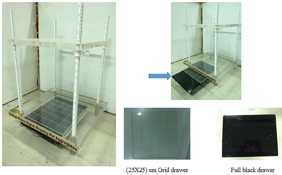
Fig. 7. Cellular phone digital mapping frame for coarse aggregate digital mapping mold for aggregate after implementation.
