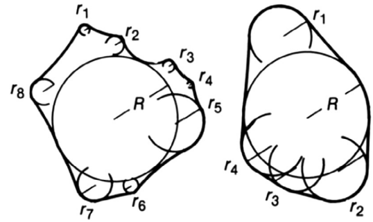
Fig. 2. Radii for the roundness.
