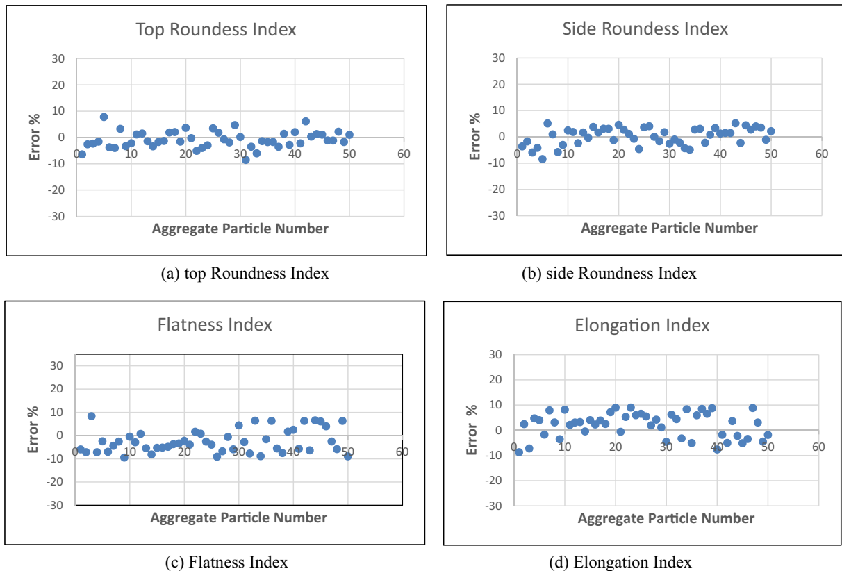
Fig. 14. Error percentages between Manual Method and the Image Processing Techniques using the ImageJ method for all aggregate particles.
