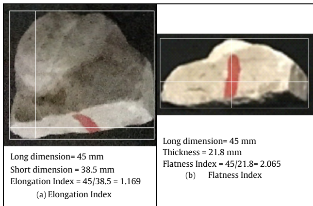
Fig. 4. Sample calculation of elongation and flatness indices.
