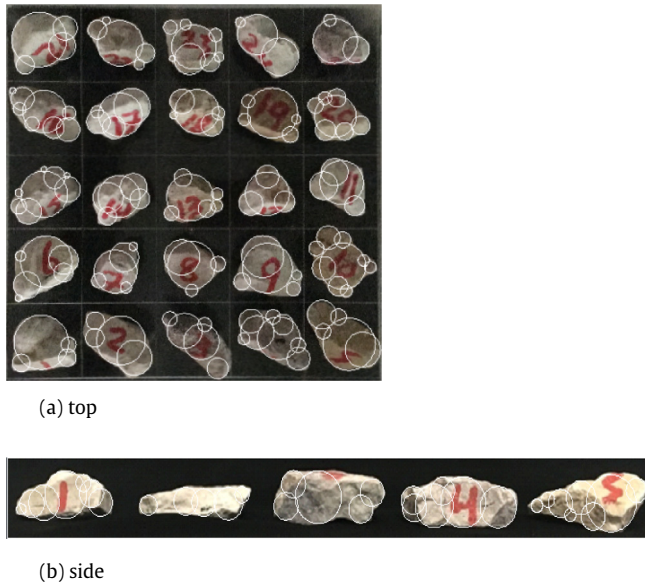
Fig. 3. Coarse aggregate Roundness Index (RI).
