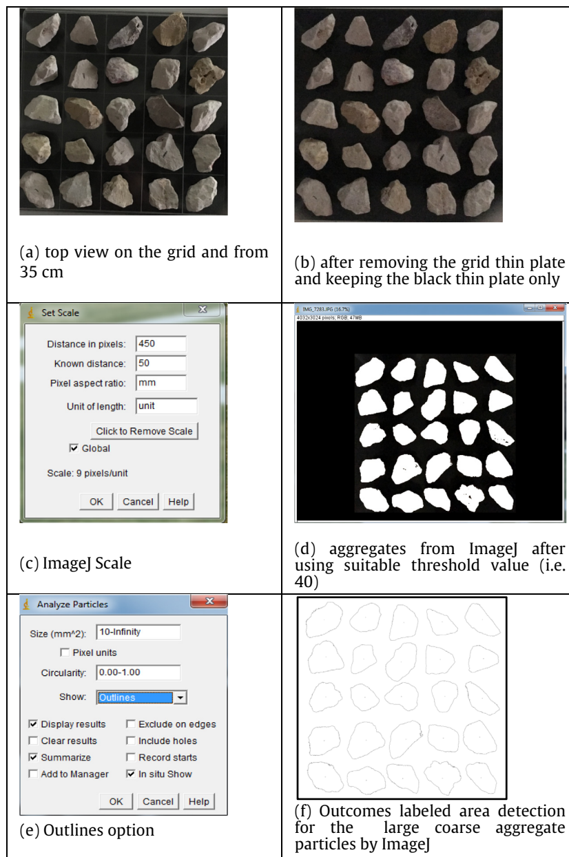
Fig. 11. The ImageJ analysis steps for the large size of coarse aggregate.
