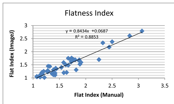
(c) Flatness Index
