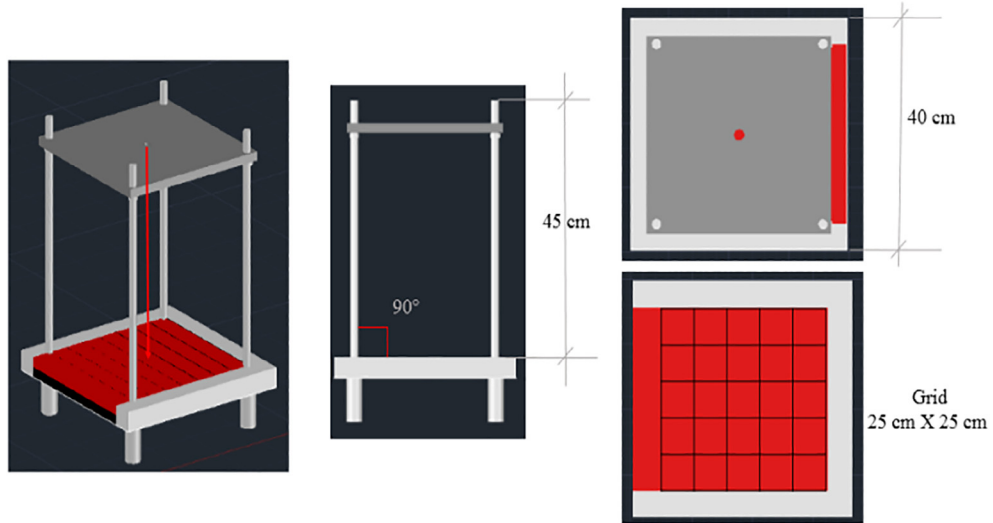
Fig. 6. AutoCAD Design of cellular phone mapping frame for Coarse Aggregates.
