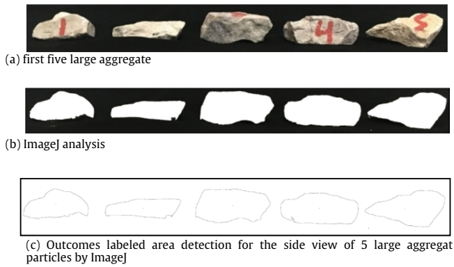
Fig. 12. ImageJ analysis for the side view of coarse aggregates.
