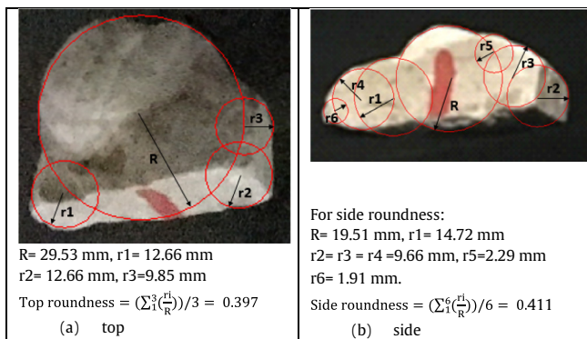
Fig. 5. Sample calculation of roundness index.
