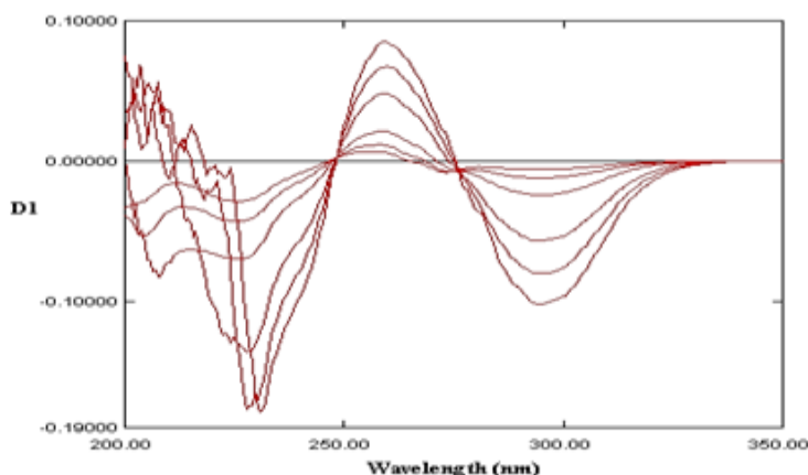
Fig. 4. First derivative spectra of mixture contain (5, 10, 20, 40, 60 and 80 \mu\text{g. mL}^{-1} ); diclofenac sodium with (5 \mu\text{g. mL}^{-1} ) nicotinamide
