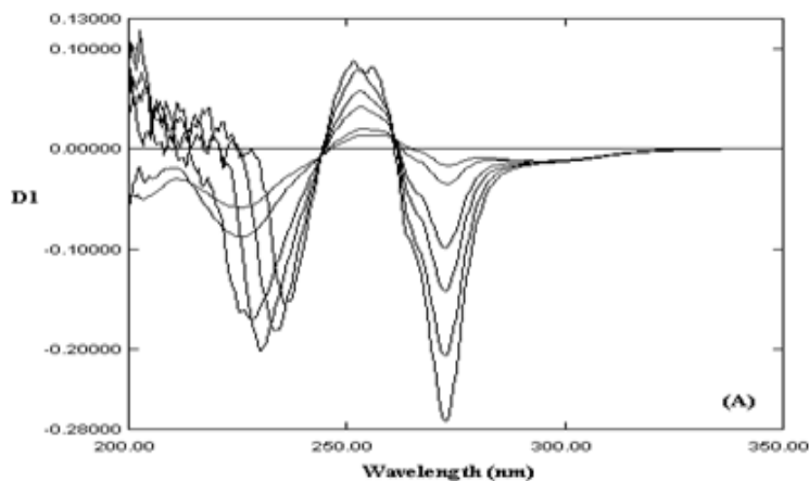
Fig. 5. First derivative spectra of mixture contain (10, 20, 50, 70, 100 and 140 \mu\text{g. mL}^{-1} ); nicotinamide with (10 \mu\text{g. mL}^{-1} ) diclofenac sodium
