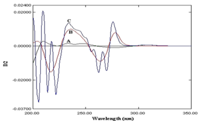
Fig. 3. 2nd derivative spectra of (A) 10 \mu\text{g. mL}^{-1} diclofenac sodium, (B) 50 \mu\text{g. mL}^{-1} nicotinamide and (C) a mixture of 10 \mu\text{g. mL}^{-1} diclofenac sodium and 50 \mu\text{g. mL}^{-1} nicotinamide
