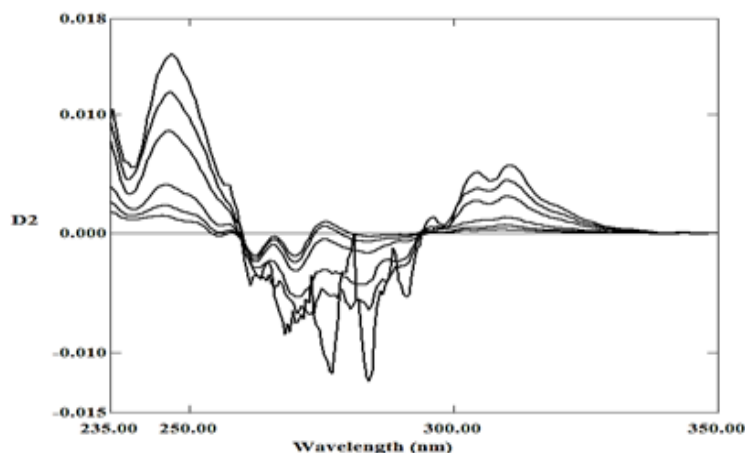
Fig. 6. Second derivative spectra of mixture contain (5, 10, 20, 40, 60 and 80 \mu\text{g. mL}^{-1} ); diclofenac sodium in existence of (5 \mu\text{g. mL}^{-1} ) nicotinamide
