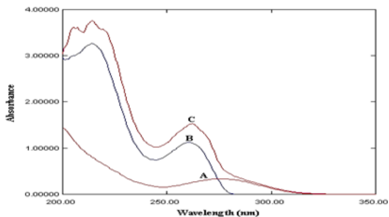
Fig. 1. Absorption spectra of: (A) 10 \mu\text{g. mL}^{-1} (DS),(B) 50 \mu\text{g. mL}^{-1} (NAM) and(C) a mixture of 10 \mu\text{g. mL}^{-1} Diclofenac sodium and 50 \mu\text{g. mL}^{-1} nicotinamide
