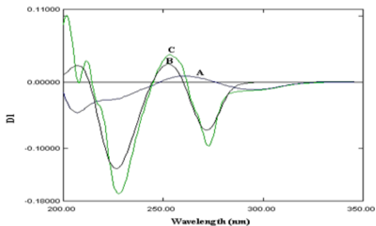
Fig. 2. 1st derivative spectra of (A) 10 \mu\text{g. mL}^{-1} Diclofenac sodium, (B) 50 \mu\text{g. mL}^{-1} nicotinamide and (C) a mixture of 10 \mu\text{g. mL}^{-1} diclofenac sodium and 50 \mu\text{g. mL}^{-1} nicotinamide
