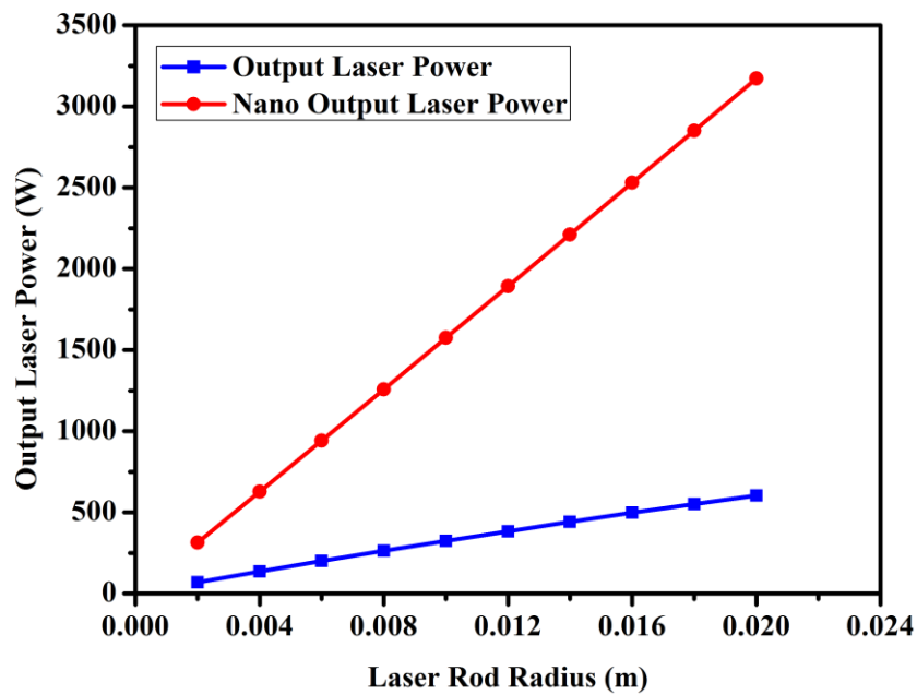
Fig. 9: The output power of the Nd:YAG laser against the radius of the rod with and without using the nano-material.
