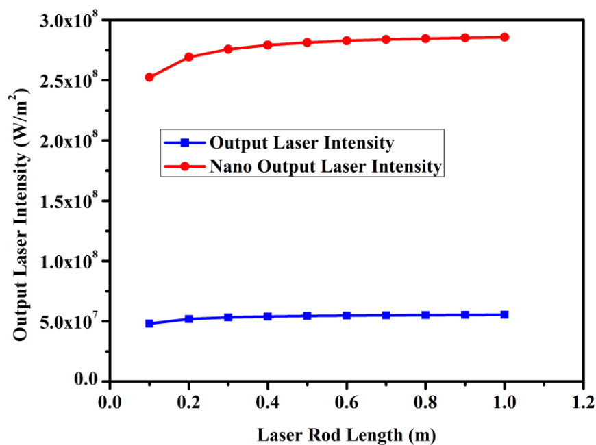
Fig. 6: The output intensity of the Nd:YAG laser against the rod length with and without using the nano-material.
