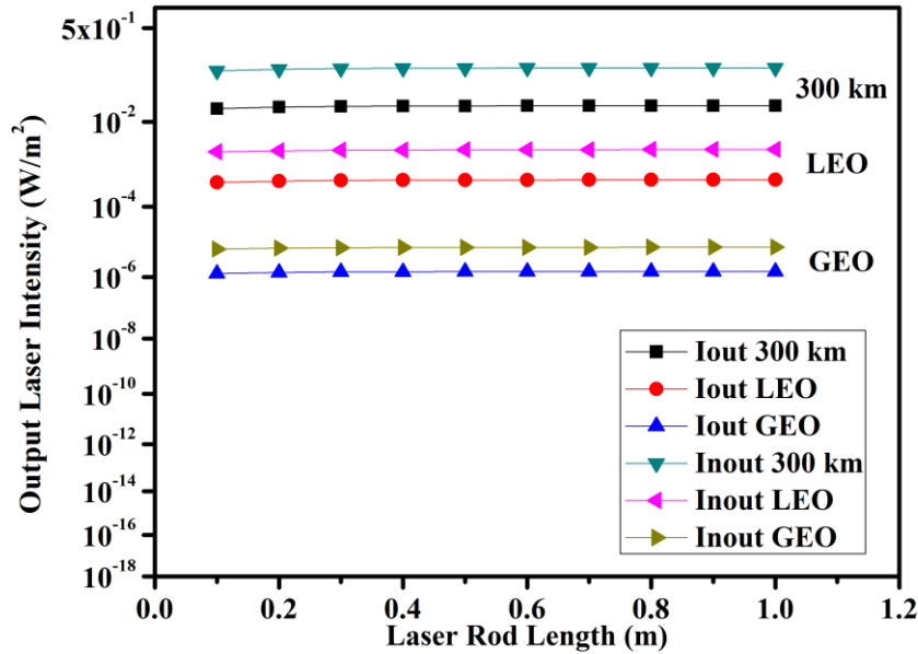
Fig. 7: A probability diagram of the output laser intensity against the length of the rod without using the nano-material on the three orbits; 300 km height, LEO and GEO respectively.
