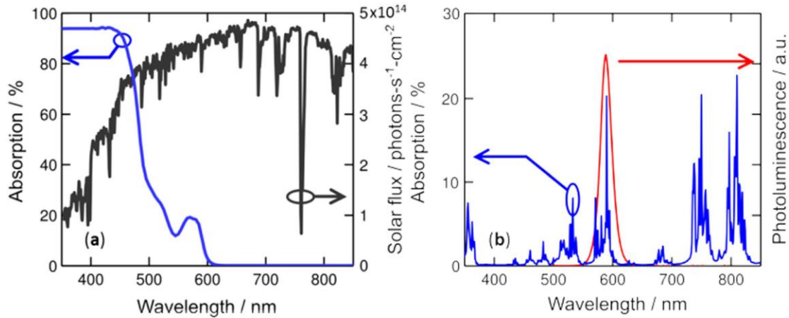
Fig. 2: (a) Absorption of the luminescent colloidal film, 10% wt. CdSe/CdZnS:PVB-CVACVAc (blue), overlaid on the AM1.5 solar flux (black). (b) The luminescence of the nanocrystal (red) is tuned to an absorption peak of the Nd 3+ :YAG (blue), for efficient waveguided luminescent pumping of optical gain media [19].
