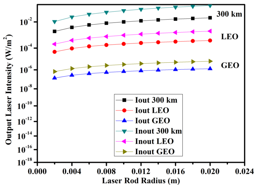
Fig. 11: A probability diagram of the output laser intensity against the radius of the rod without using the nano-material on the three orbits; 300 km height, LEO and GEO respectively.
