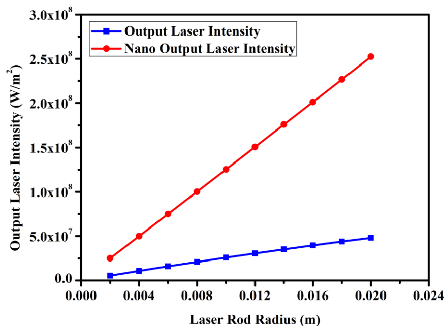
Fig. 10: The output intensity of the Nd:YAG laser against the radius of the rod with and without using the nano-material.
