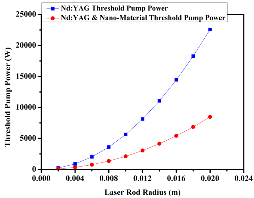
Fig. 8: The threshold pumping power of the Nd:YAG laser against the radius of the rod with and without using the nano-material.
