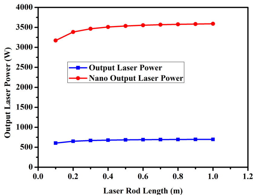
Fig. 5: The output power of the Nd:YAG laser against the length of the rod with and without using the nano-material.
