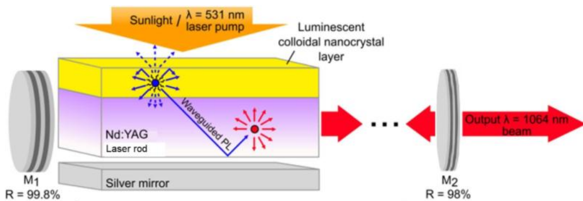
Fig. 3: The design of the laser cavity.
