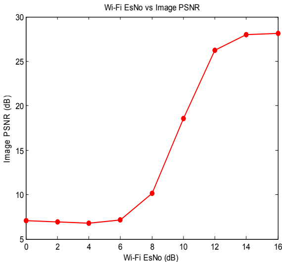
Figure 18: PSNR Result On Data Transmission Simulation Using Proposed Image Compression On Grayscale Radiography Image
