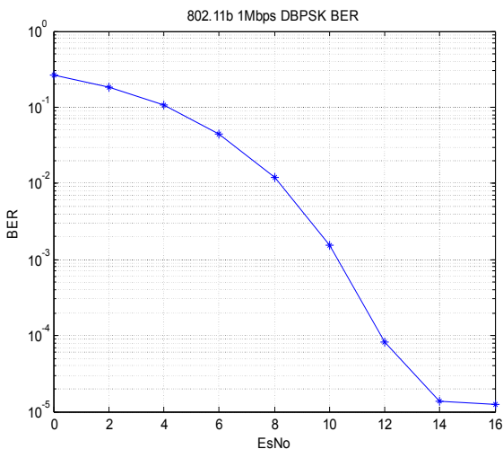
Figure 19: BER Result On 1 Mbps Wi-Fi Transmission Simulation Using Proposed Image Compression On Grayscale Radiography Image
