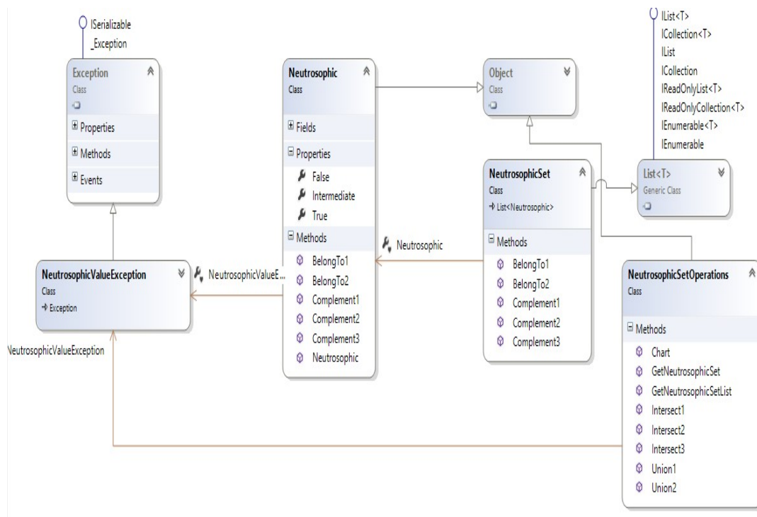
Figure 6. Neutrosophic Package Class Diagram
