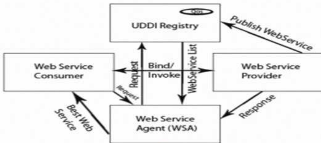
Figure 4: Web service discovery Framework
