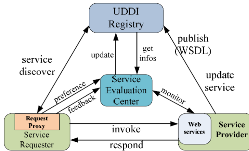
Figure 19: Extended Service Discovery Model
