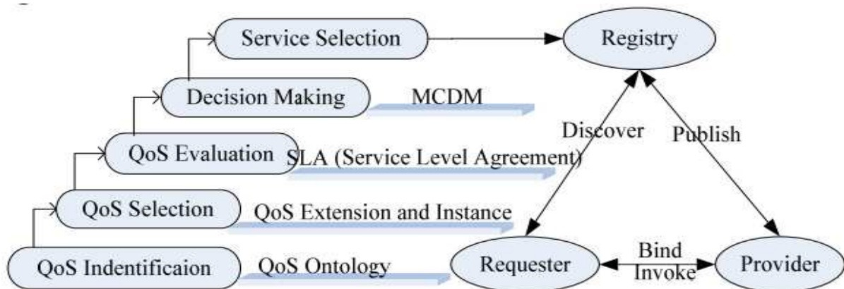
Figure 3: The framework of Web service selection process
