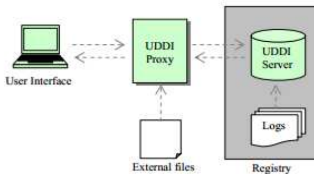
Figure 8: Proposed model architecture
