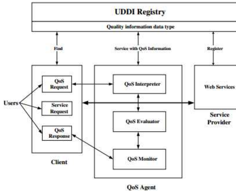
Figure 16: Web service with QoS agent architecture
