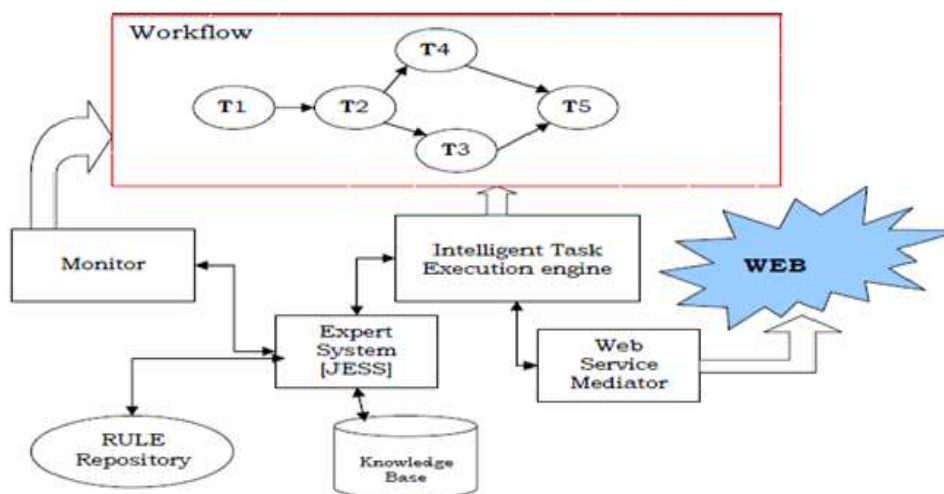
Figure 11: The Web Architecture
