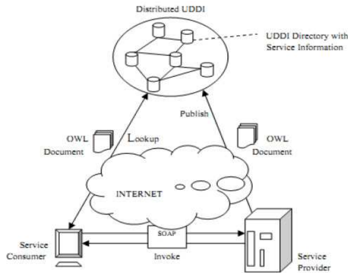
Figure 7: Service Discovery model Distributed UDDI
