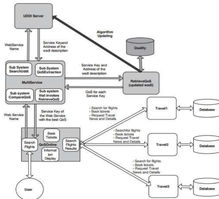
Figure 15: The general architecture of the proposed model
