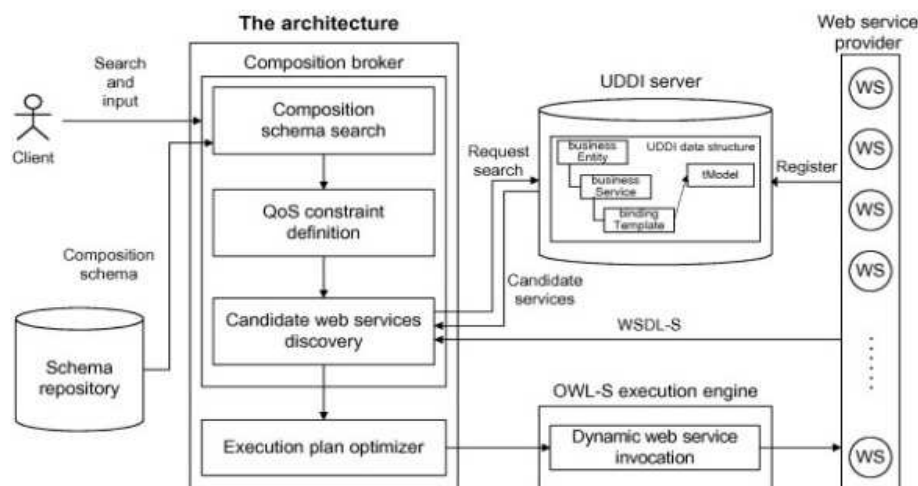
Figure 14: QoS-oriented web service composition planning architecture
