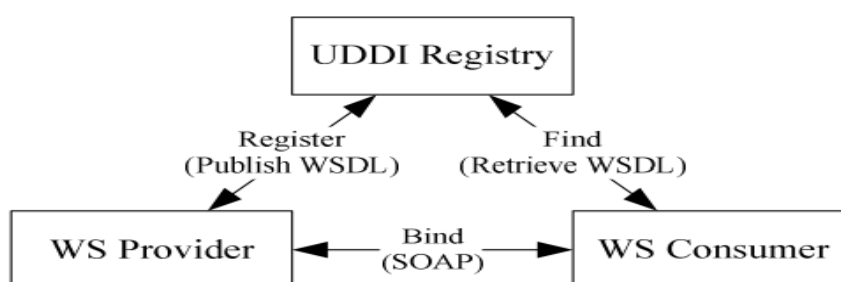
Figure 2: Register-find-bind model for Web Services discovery
