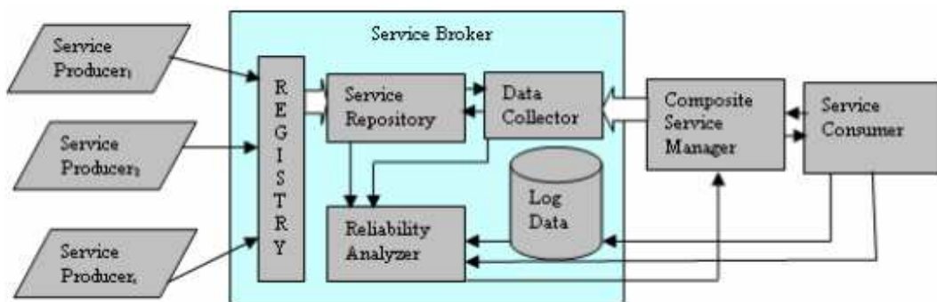
Figure 13: Framework model for Reliability Evaluation in Composite Web Service
