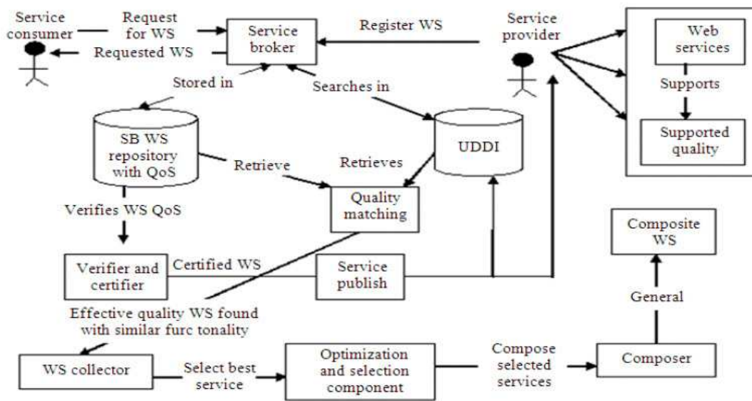
Figure 12: The detailed QoS broker based- process model for dynamic WS composition
