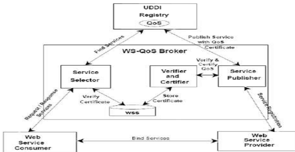
Figure 9: Architecture for WS-QoS Broker
