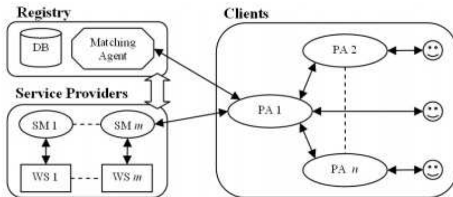
Figure 6: Web service Discovery Model
