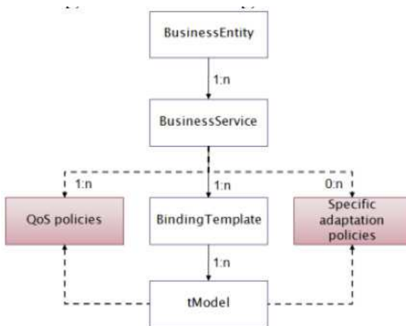
Figure 18: Extended UDDI information model
