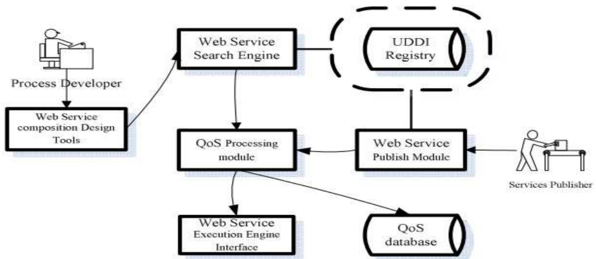
Figure 5: Architecture of the framework
