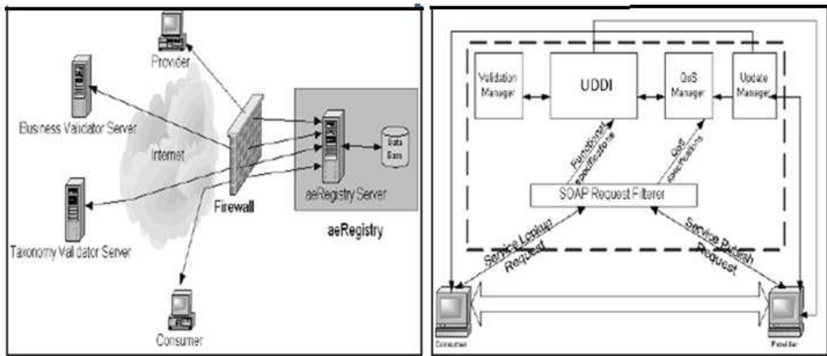
Figure 10: Web Service based framework for adaptive workflow management
