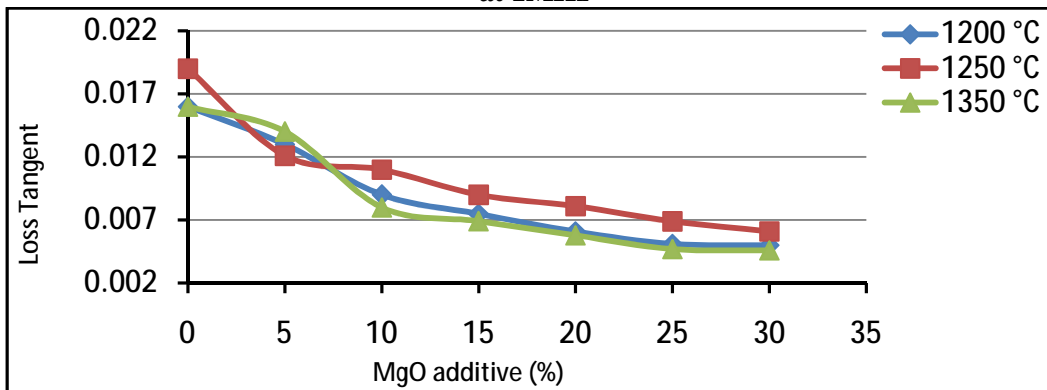
Figure (6) Loss tangent of electrical porcelain against MgO content at different temperature at 1MHz
