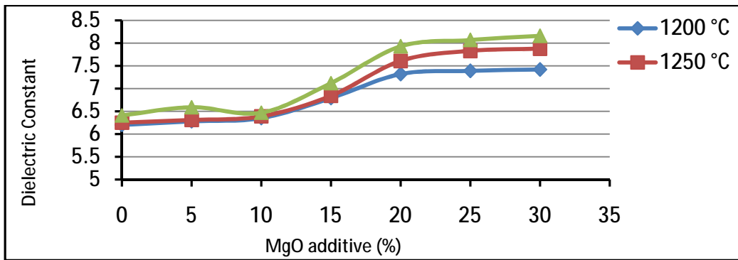
Figure (5) Dielectric constant of electrical porcelain against MgO content at 1MHz
