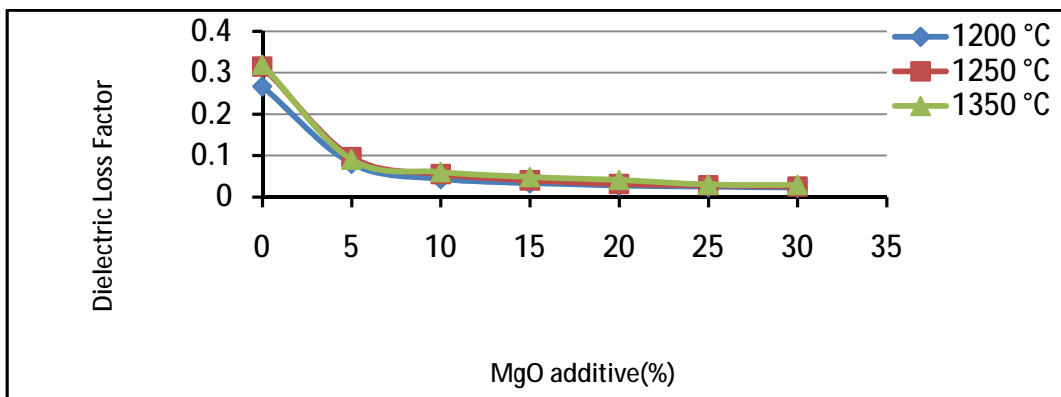
Figure(7) Dielectric loss factor of electrical porcelain against MgO content at 1MHz
