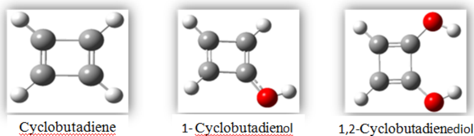
Fig. 1: The schematic representation for cyclobutadienes its group.
