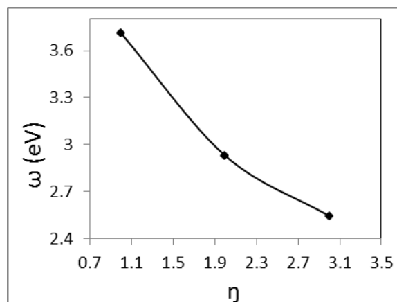
Fig. 4: Relationship between electrophilicity and the number of the molecules.
