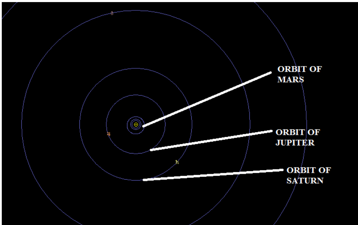
FIG. THE ORBIT OF THE EARTH IS THE NEXT AFTER THE MARS ORBIT INTO THE SUN, SO THE MID. POINT ON THE RADIUS OF THE THRONE OF ALLAH IS NEAR THE JUPITER ORBIT [2].
