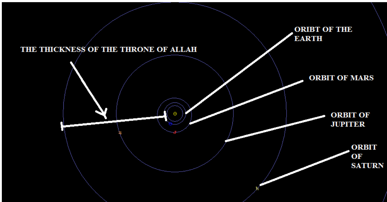
FIG. THE THICKNESS OF THE THRONE OF ALLAH IN THIS SOLAR SYSTEM
