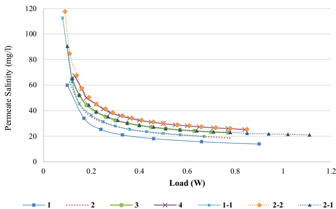
Fig. 5. Permeate salinity versus load power at different design configurations using TW30-4040 under feed salinity of 2000 mg/l.
