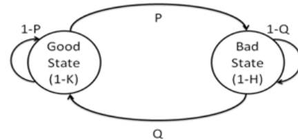
Figure 5. Markov probability model.
