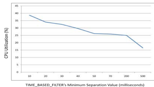
Figure 8. CPU Utilization.
