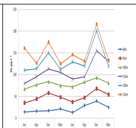
Fig. 8: Zn µg L -1 values for EL-Serw drainage water.
