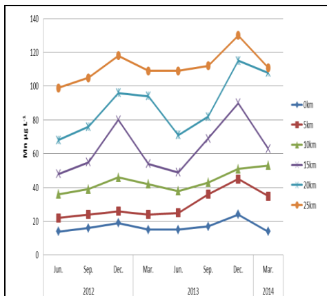
Fig. 5: Mn µg L -1 values for EL-Serw drainage water.
