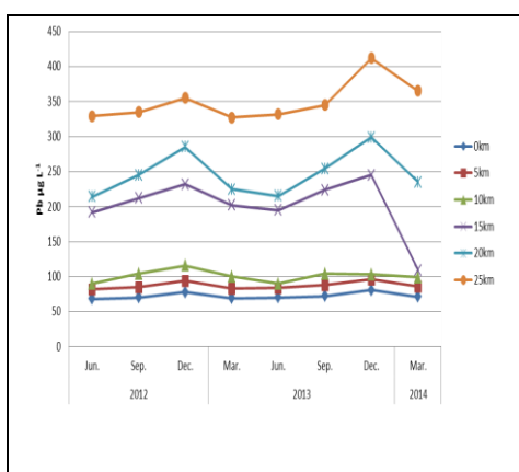
Fig. 7: pb µg L -1 values for EL-Serw drainage water.
