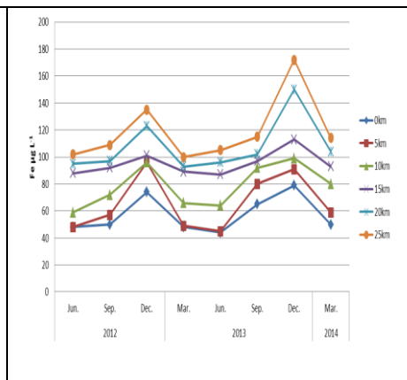
Fig. 6: Fe µg L -1 values for EL-Serw drainage water.
