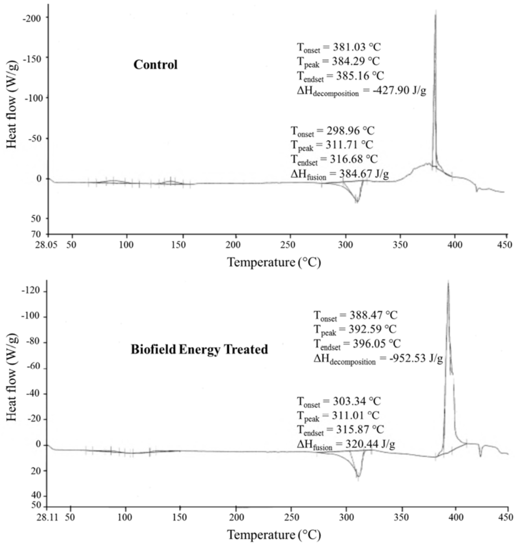
Figure 4. DSC thermograms of the control and Biofield Energy Treated zinc chloride.
