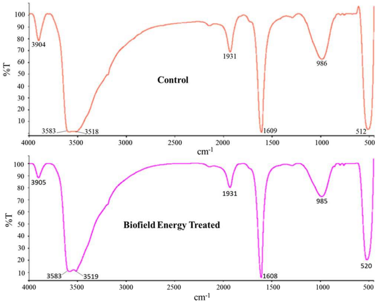
Figure 2. FT-IR spectra of the control and Biofield Energy Treated zinc chloride.
