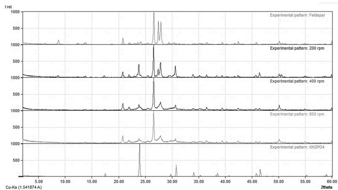
Figure 1. An XRD pattern of the Feldspar-KH 2 PO 4 sample mixture was milled at varying mill rotational speeds for 120 min.
