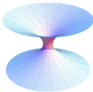
SCHWARZSCHILD WORMHOLE
